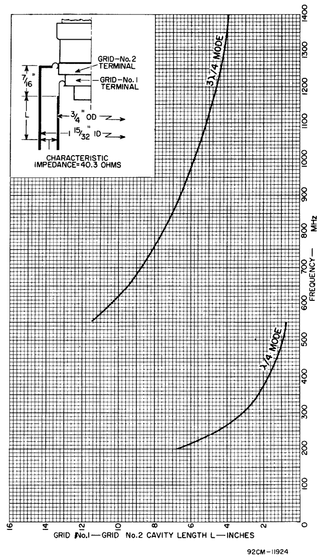
Figure 11 - Grid No. 1 - Grid No.2 Tuning Curves.
